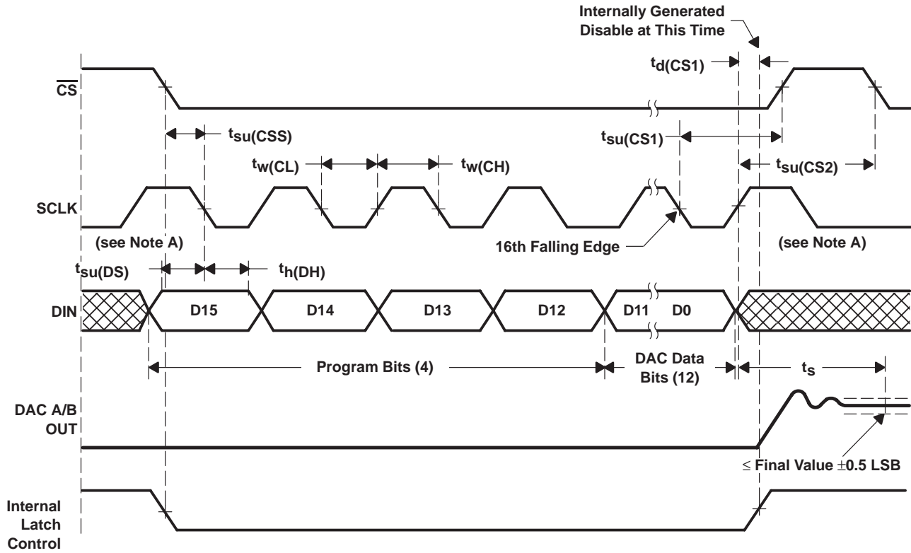
Figure 2. Timing Diagram for TLC5618A Only
